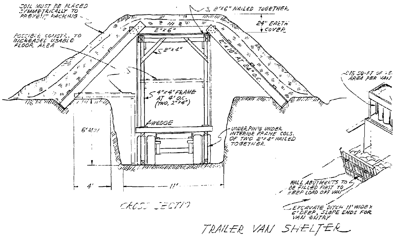
Fig. A-12.1. Trailer Van Shelter, Pictorial View and Sections.
